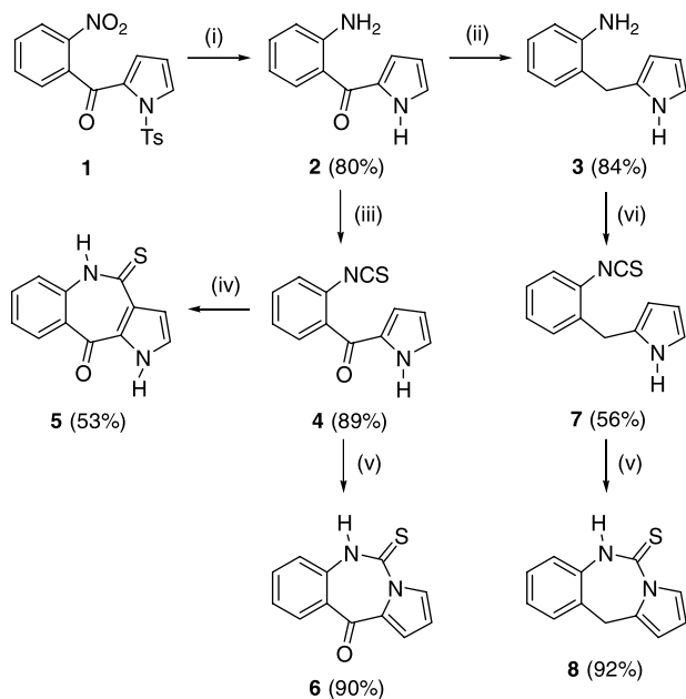
Scheme 1. Reagents and conditions: (i) (a) \text{H}_2 , 5% Pd-C, MeOH, rt, 8 h; (b) aq 2 N NaOH, MeOH, reflux, 5 h; (ii) \text{NaBH}_4 , IPA, reflux, 24 h; (iii) \text{CSCl}_2 , toluene, \text{Et}_3\text{N} , rt, 1 h; (iv) \text{AlCl}_3 , \text{MeNO}_2 , rt, 6.5 h; (v) \text{K}_2\text{CO}_3 , DMF, rt, 3 h; (vi) \text{CSCl}_2 , toluene, \text{Et}_3\text{N} , -45^\circ\text{C} , 5 min.
