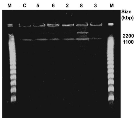
Figure 1. Detection of intracellular DNA cleavage in Jurkat cells treated with heterocycles 2 , 3 , 5 , 6 , and 8 . Cells ( 1 \times 10^6 /ml) were treated with 1 \mu\text{M} of each heterocycle 2 , 3 , 5 , 6 , and 8 at 37^\circ\text{C} for 20 h. Cells, prepared as agarose plugs, were lysed and subjected to pulsed field gel electrophoresis through a 1% agarose gel. C, control; M, size marker DNA.
